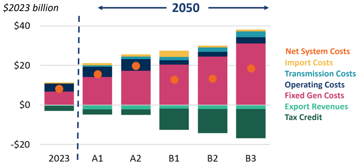
FIGURE 20: SPP ANNUALIZED GENERATION AND TRANSMISSION COSTS (2023 AND 2050) (inflation adjusted, in $2023 billion/year) 16
