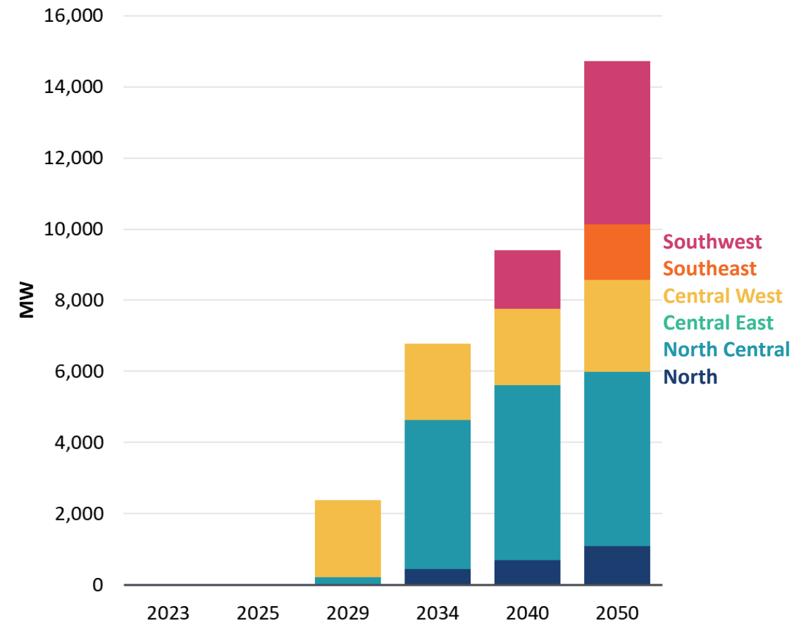
SPP Cumulative Economic Interzonal Transmission Expansion (MW of added zonal import/export capability, Scenario B2)
