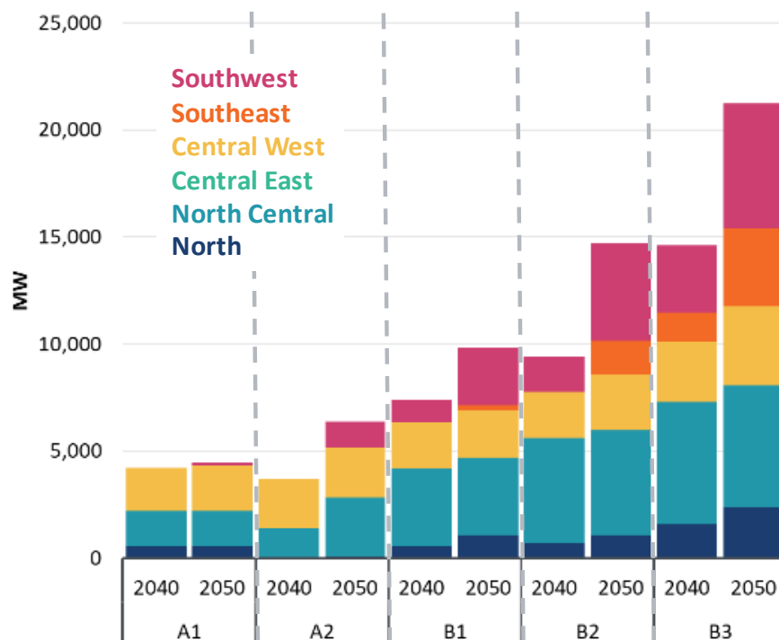
FIGURE 9: TOTAL SPP INTERZONAL TRANSMISSION EXPANSIONS ACROSS FERNs SCENARIOS (MW OF ADDED ZONAL IMPORT/EXPORT CAPABILITY BY 2040 AND 2050)
