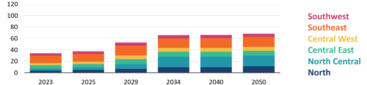
SPP Battery Storage Capacity (GW)
