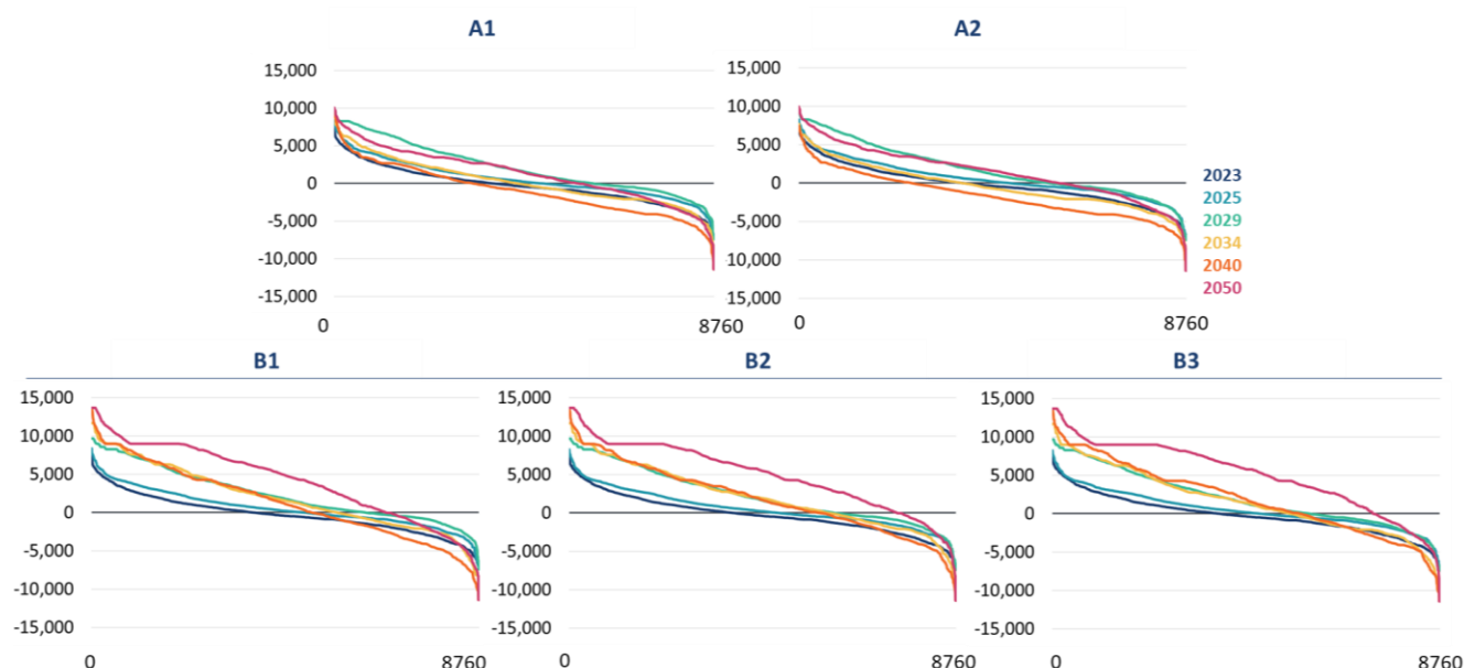
FIGURE 10: SPP NET IMPORTS AND EXPORTS WITH NEIGHBORING REGIONS (MW) (POSITIVE = NET FLOW OUT OF SPP; NEGATIVE = NET FLOW INTO SPP) 11
