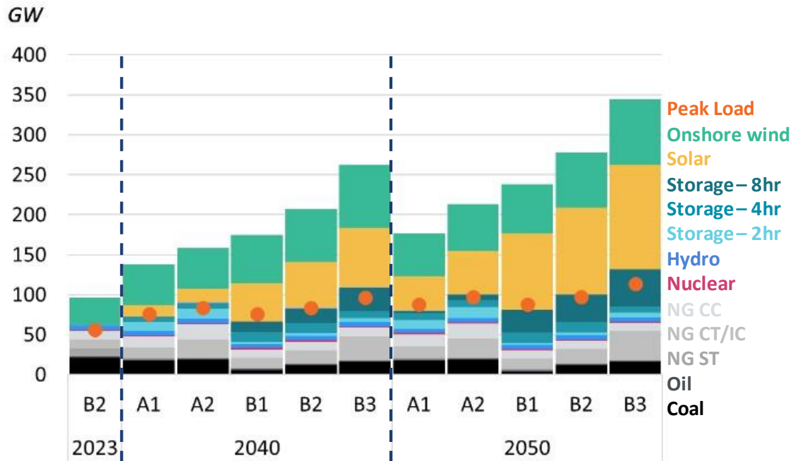
FIGURE 6: SPP TOTAL INSTALLED GENERATION CAPACITY ACROSS FERNs SCENARIOS
