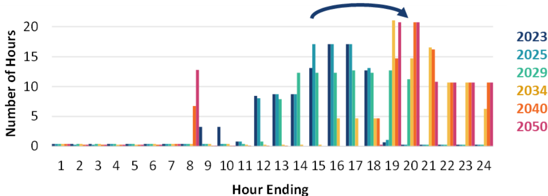
FIGURE 14: TOP 100 RESOURCE ADEQUACY RISK HOURS BY HOUR (SCENARIO B2)
