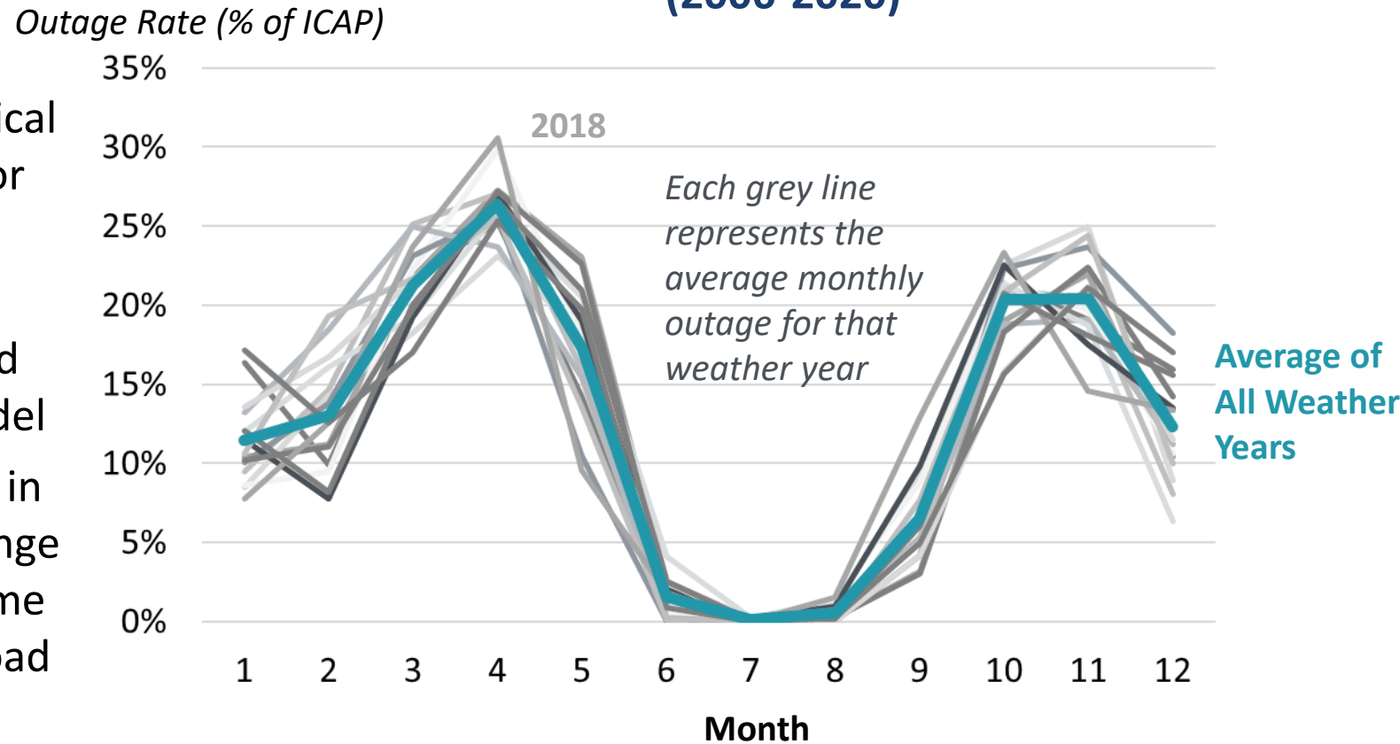
Monthly Average SPP Generation Outage Rate (2006-2020)
