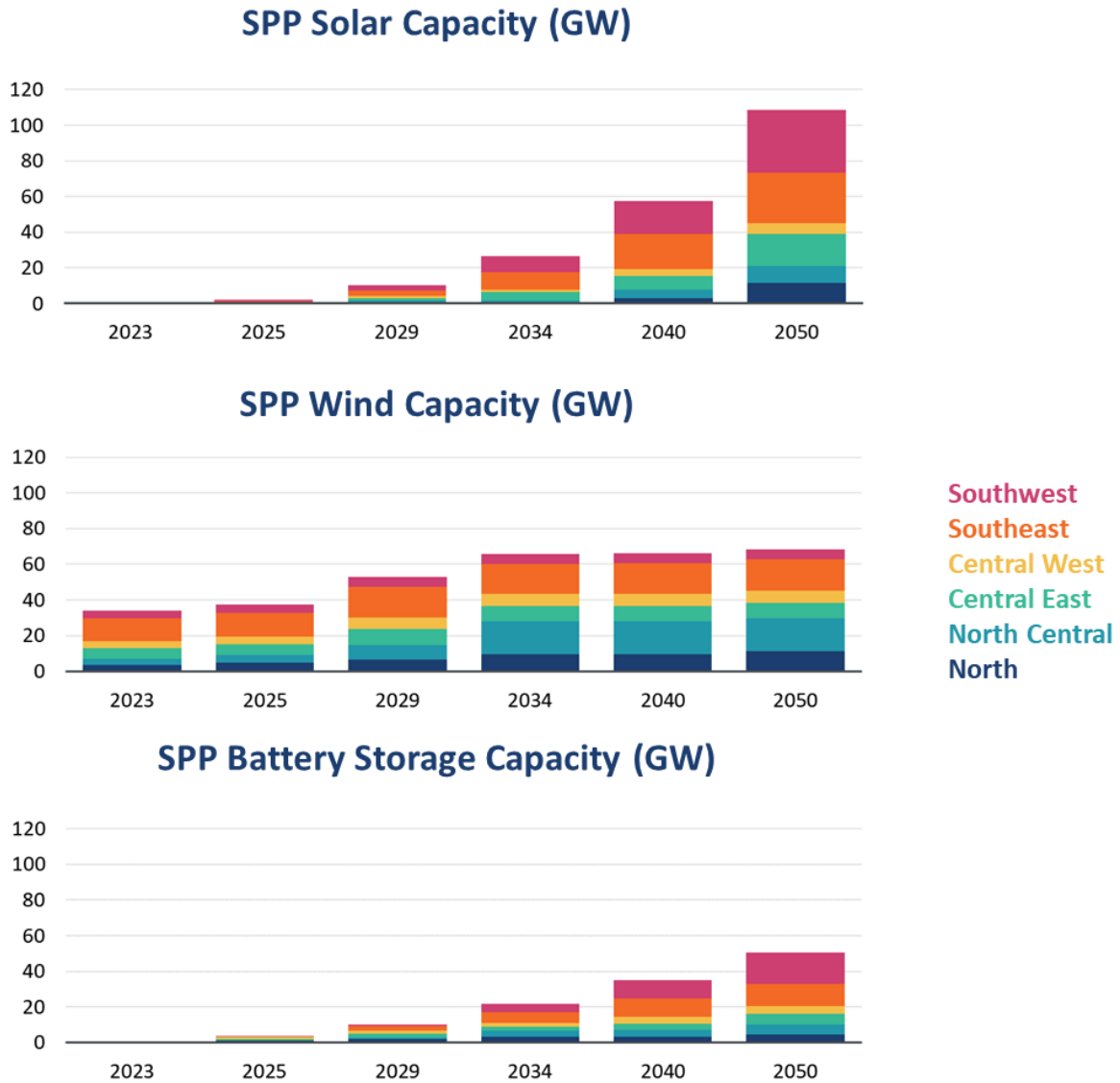
FIGURE 7: TOTAL INSTALLED RENEWABLE GENERATION AND STORAGE BY ZONE (SCENARIO B2)
