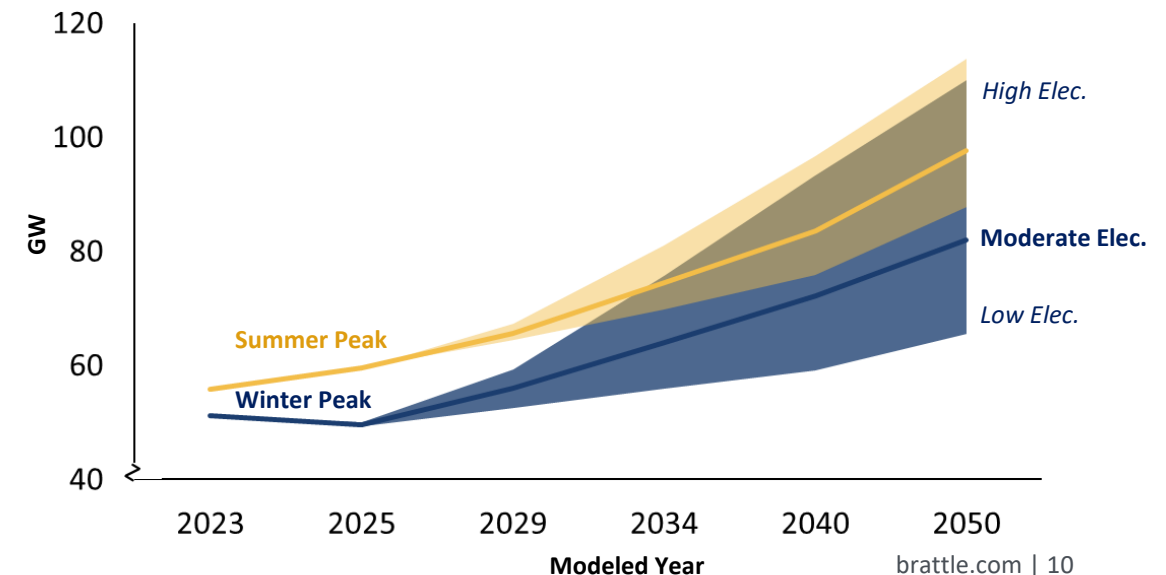
SPP Peak Load for FERNS Scenarios
