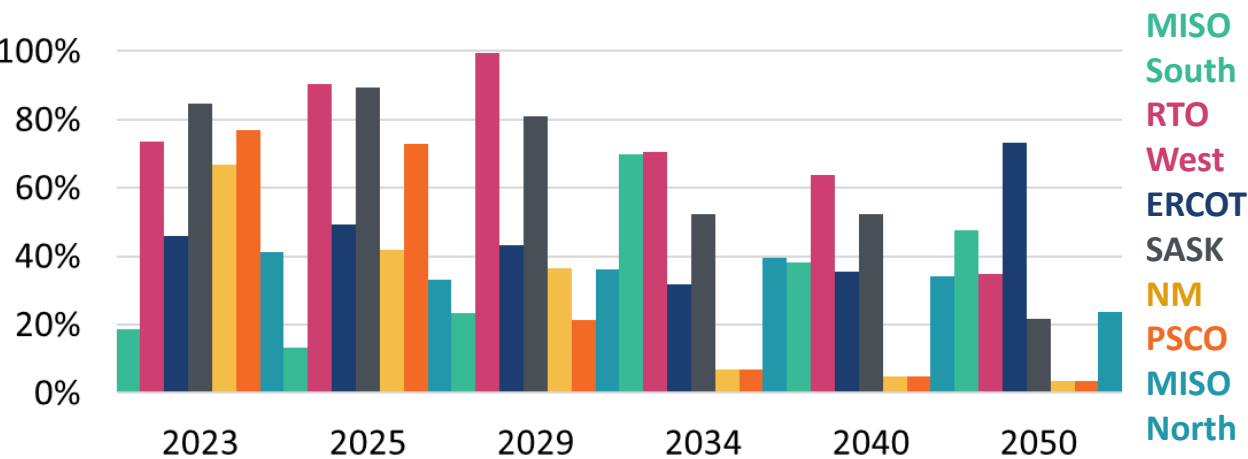
Implied “Proxy ELCCs” of Non-firm Energy Imports over Interties with Neighboring Regions (Scenario B2)
