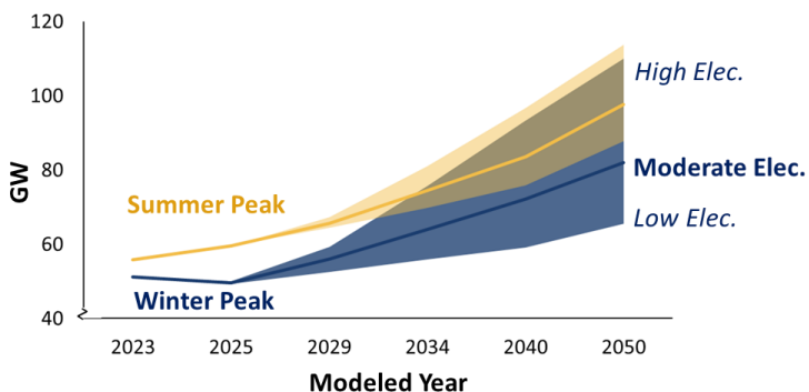
FIGURE ES-2: SPP PEAK LOAD SCENARIOS
