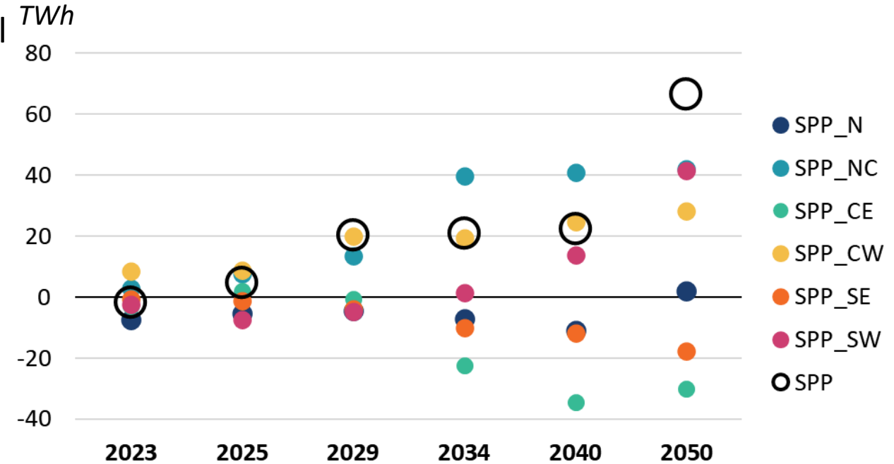
SPP Annual Internal Interface Flows
