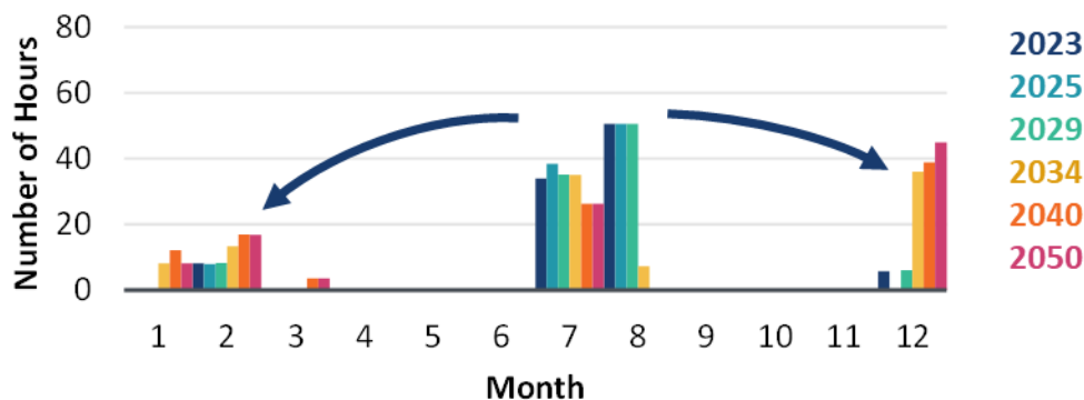
FIGURE 13: TOP 100 RESOURCE ADEQUACY RISK HOURS BY MONTH (SCENARIO B2)
