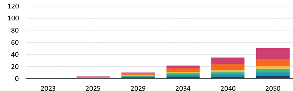
SPP Battery Storage Capacity (GW)
