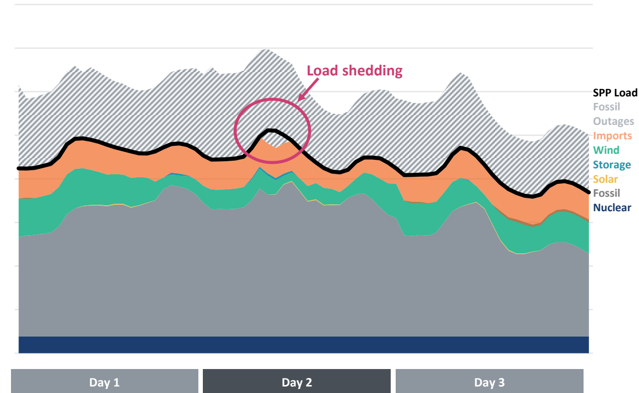
SPP Winter Risk Period (Three-day period in 2023)
