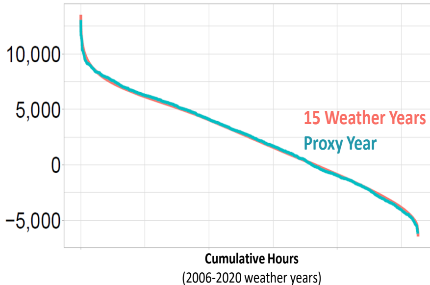
FIGURE 4: SPP CENTRAL-EAST NET LOAD DURATION CURVE FOR 2029 (MW) (Adjusted for renewable generation and temperature-correlated generation outages)
