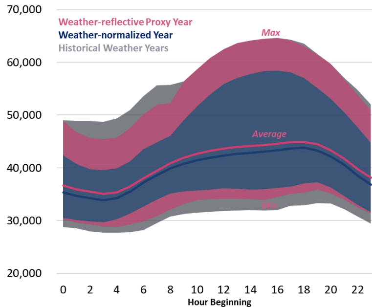
FIGURE 3: RANGE OF DAILY SPP-WIDE 24-HOUR GROSS LOADS IN 2029 (MW)
