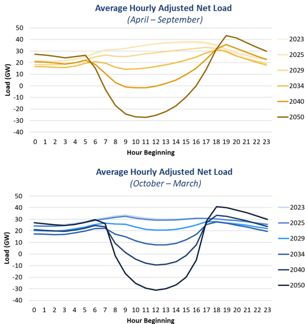
FIGURE 11: SPP'S AVERAGE HOURLY "ADJUSTED NET LOAD" FOR SUMMER AND WINTER DAYS 13
