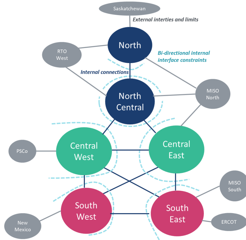
FIGURE 1: FERNS ZONAL TOPOLOGY
