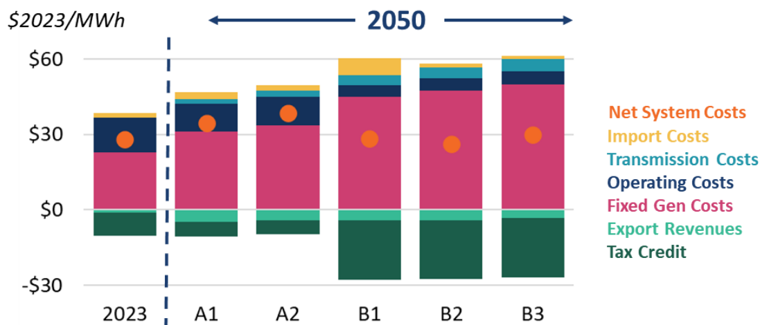
FIGURE 21: SPP GENERATION AND TRANSMISSION COSTS IN $/MWH (2023 AND 2050) (inflation adjusted, in 2023 dollars)
