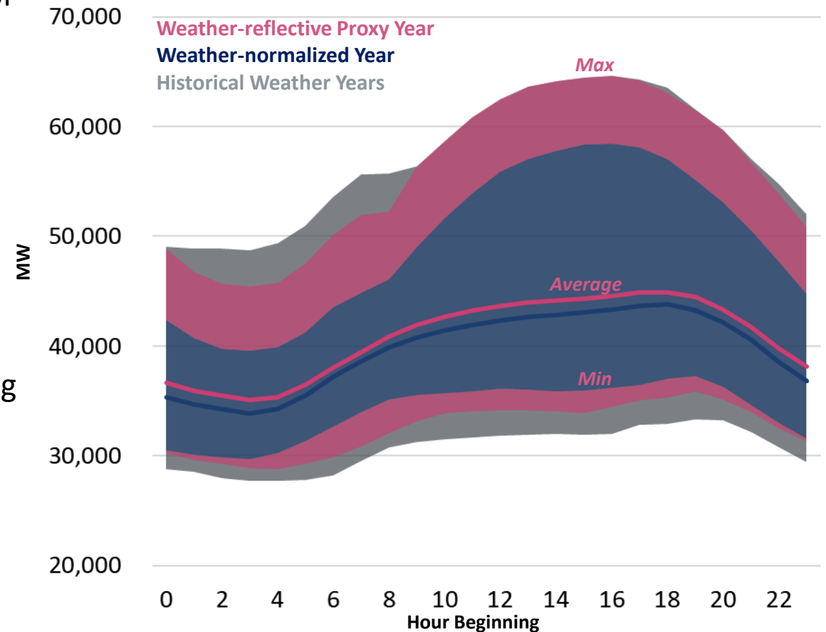
SPP-Wide 24-Hour Load Shape (2029, Moderate Scenario)
