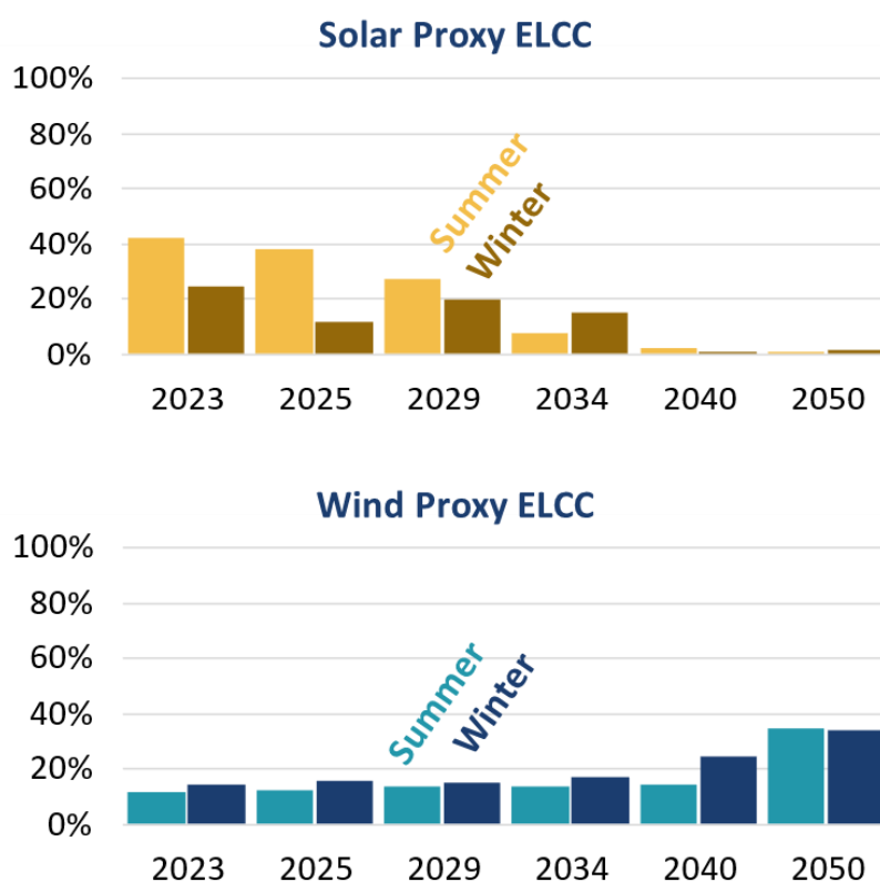
FIGURE 15: PROXY SEASONAL ELCC VALUES FOR WIND AND SOLAR RESOURCES (SCENARIO B2)
