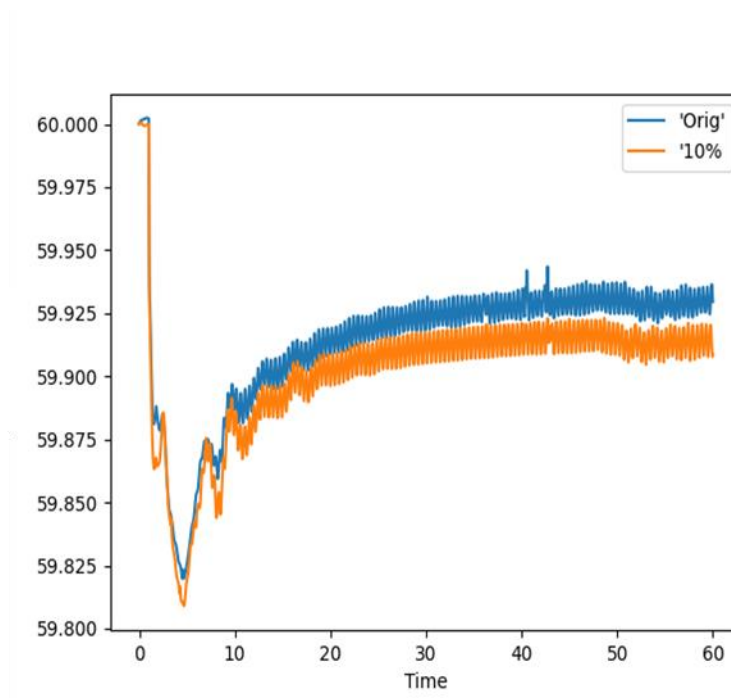
Figure 6.3-5: 2034 Scenario 3: System Frequency Response for all CAISO BESS at 10% Headroom vs Original case (SC2)
